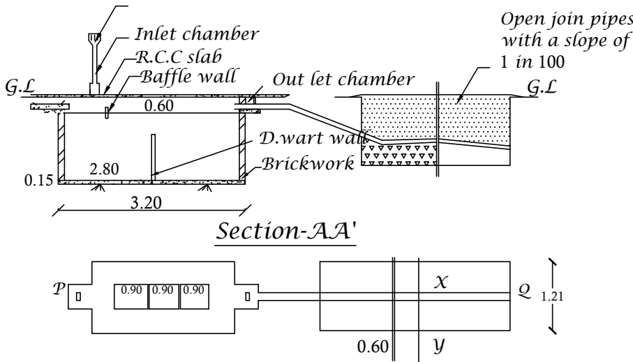
Septic Tank Dispersion Trench
