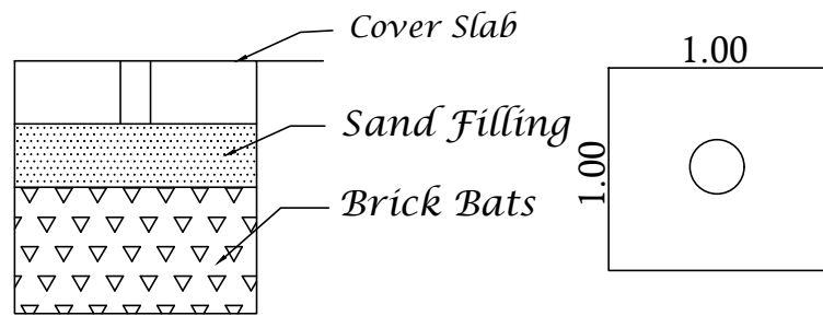
Rain Water Harvesting Details
