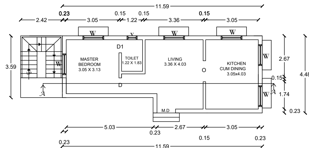
Pro.Ground Floor
