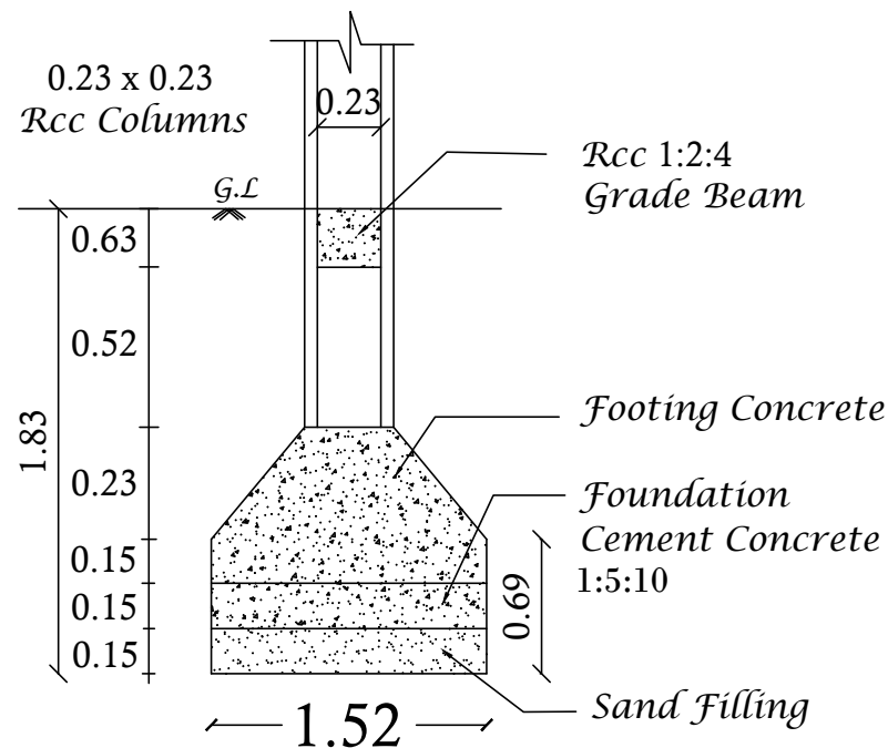
Foundation Details
