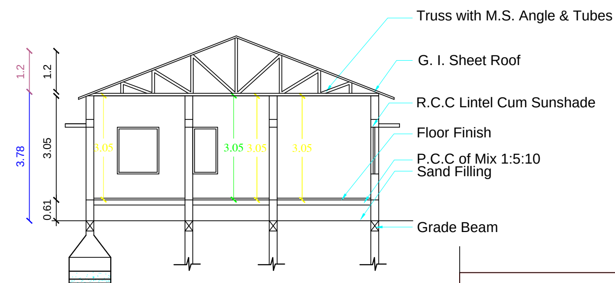
SECTION ON "PQ"
