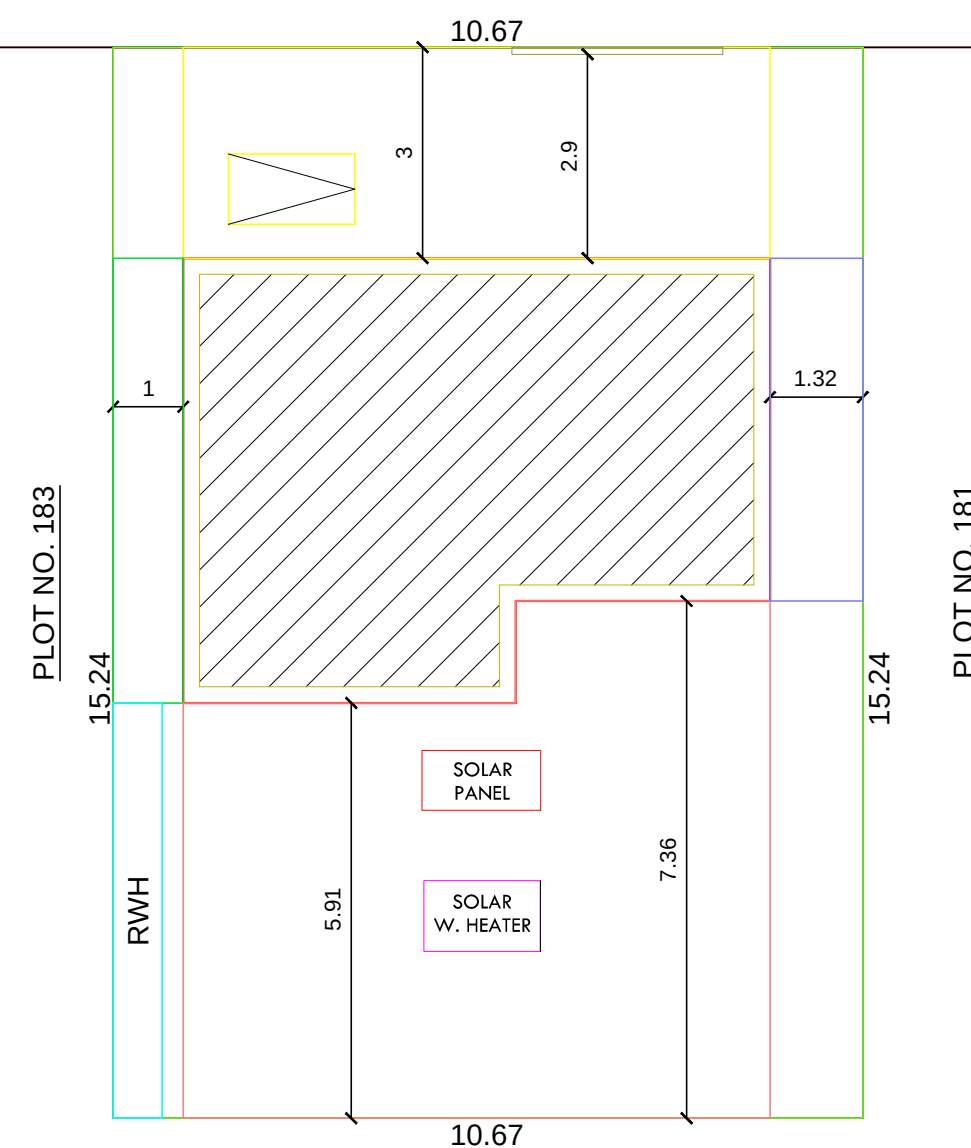
SITE PLAN
