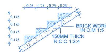
STAIRCASE DETAILS NOT TO SCALE
