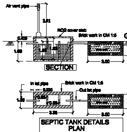
SEPTIC TANK DETAILS PLAN
