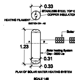
PLAN OF SOLAR WATER HEATING SYSTEM SCALE 1:50
