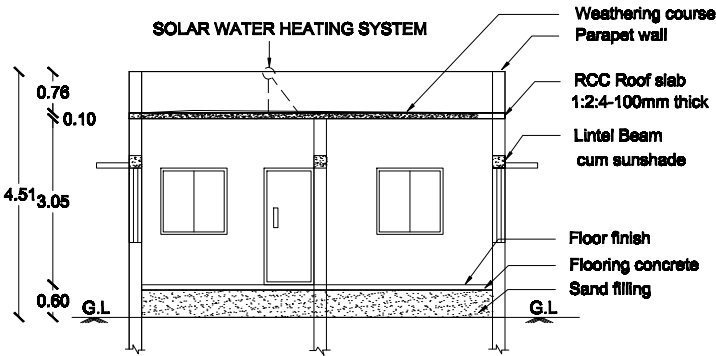
SECTION ON MK
