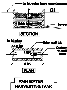
RAIN WATER HARVESTING TANK
