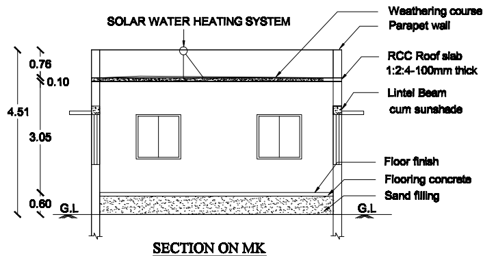
SECTION ON MK
