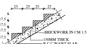
DETAIL OF THE STEPS
