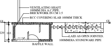
SECTION OF SEPTIC TANK
