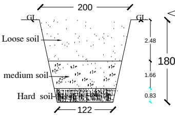
Trail pit details
