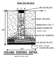
COLUMN FOOTING DETAIL
