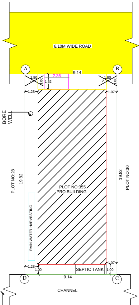
KEY PLAN
