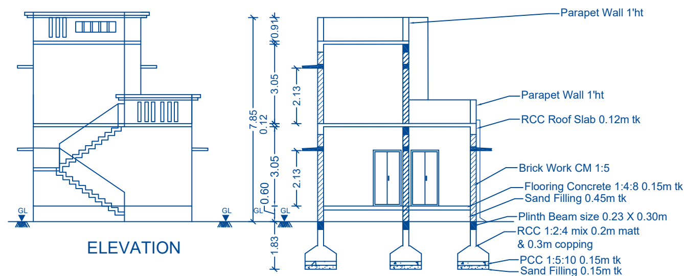
SECTION-AB
