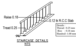
STAIRCASE DETAILS NTS
