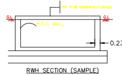
RW SECTION (SAMPLE)
