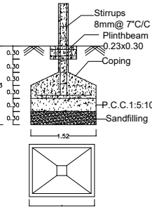
Foundation Details
