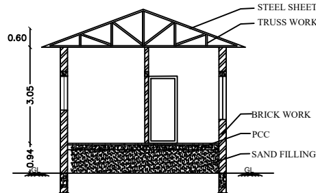
SECTION ON HH
