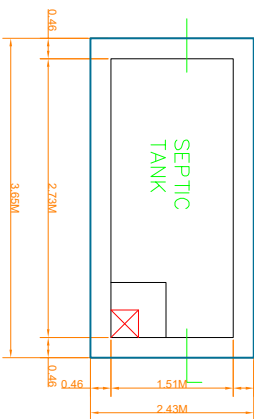
PLAN OF SEPTIC TANK SCALE 1"=2'0"
