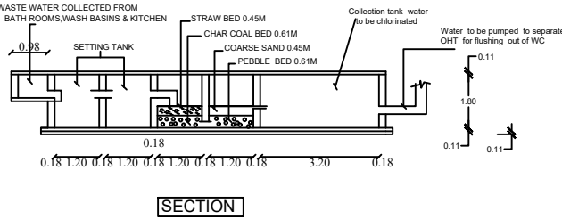
SECTION
