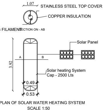
PLAN OF SOLAR WATER HEATING SYSTEM SCALE 1:50
