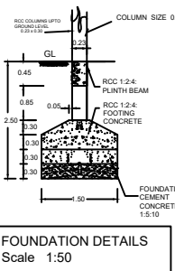
FOUNDATION DETAILS Scale 1:50
