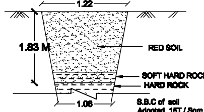
TRIAL PIT DETAILS NOT TO SCALE
