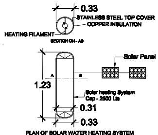
PLAN OF SOLAR WATER HEATING SYSTEM SCALE 1:50
