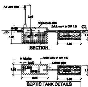
SEPTIC TANK DETAILS PLAN
