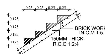
STAIRCASE DETAILS NOT TO SCALE
