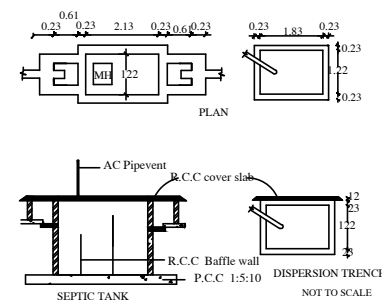
SEPTIC TANK SECTION NOT TO SCALE
