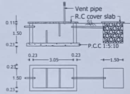
SEPTIC TANK & D-TRENCH DETAILS
