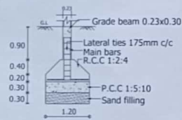
FOOTING DETAILS SCALE 1:50
