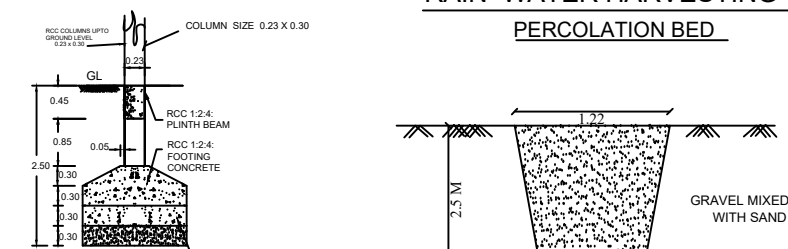
TRIAL PIT DETAILS
