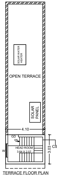
TERRACE FLOOR PLAN
