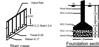
Stair case
