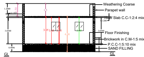
CROSS SECTION ON AB
