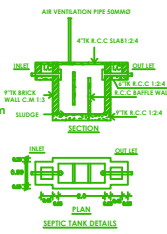
SEPTIC TANK DETAILS
