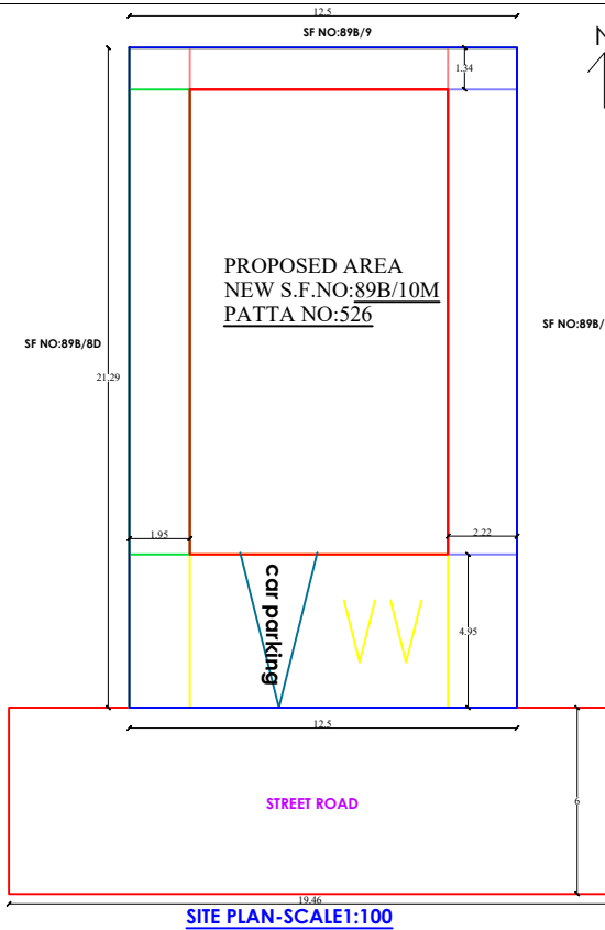
SITE PLAN-SCALE:1:100
