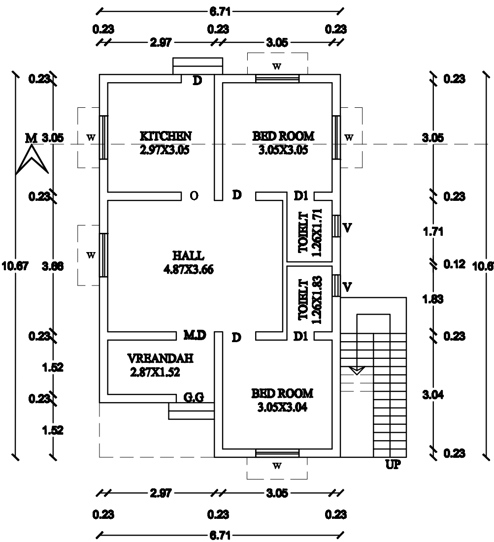
EXI-GROUND FLOOR PLAN
