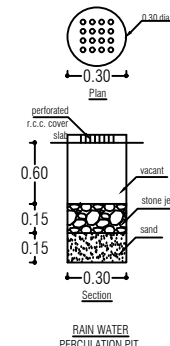
RAIN WATER PERCOLATION PIT
