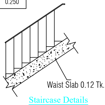
Staircase Details
