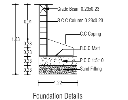
Foundation Details
