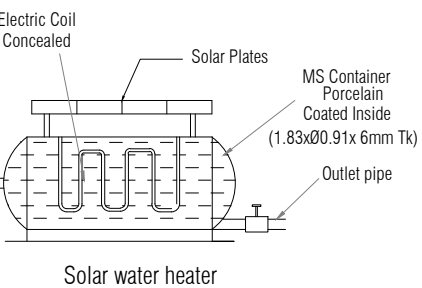
Solar water heater
