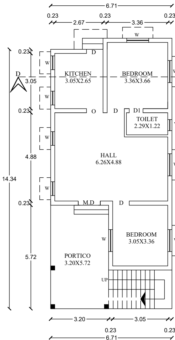
PRO - GROUND FLOOR PLAN
