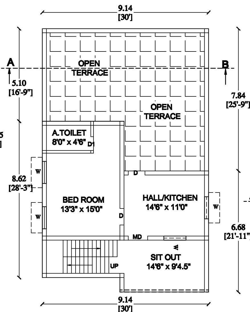
PRO.FIRST FLOOR
