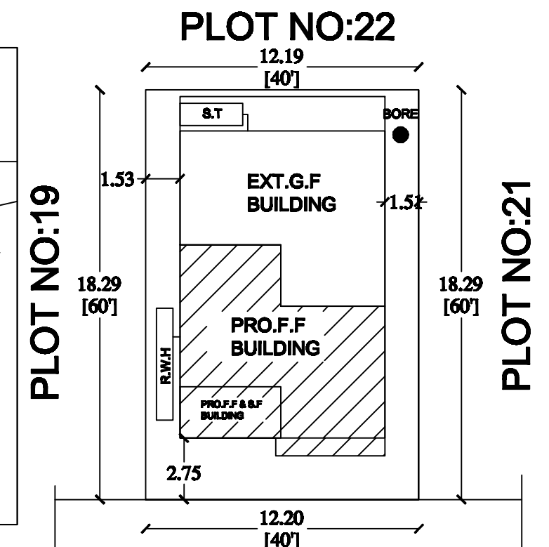
VALAPAKUDI SALAI SITE PLAN (SCALE 1:200)
