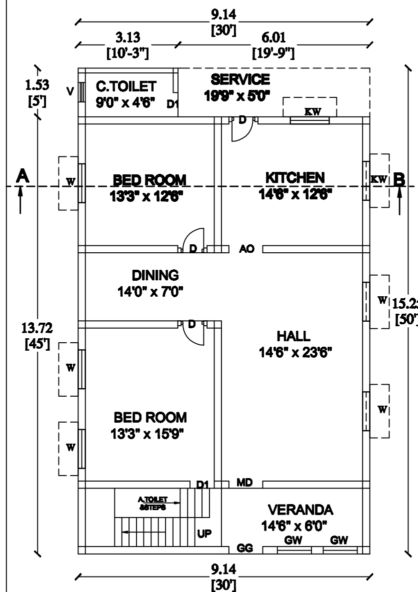
EXT.GROUND FLOOR
