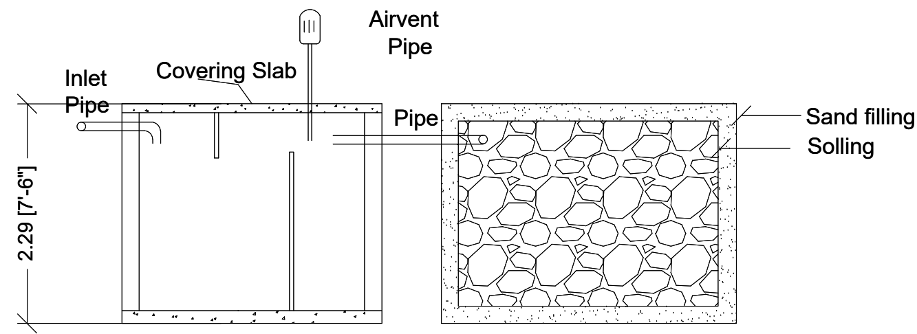
SECTION
