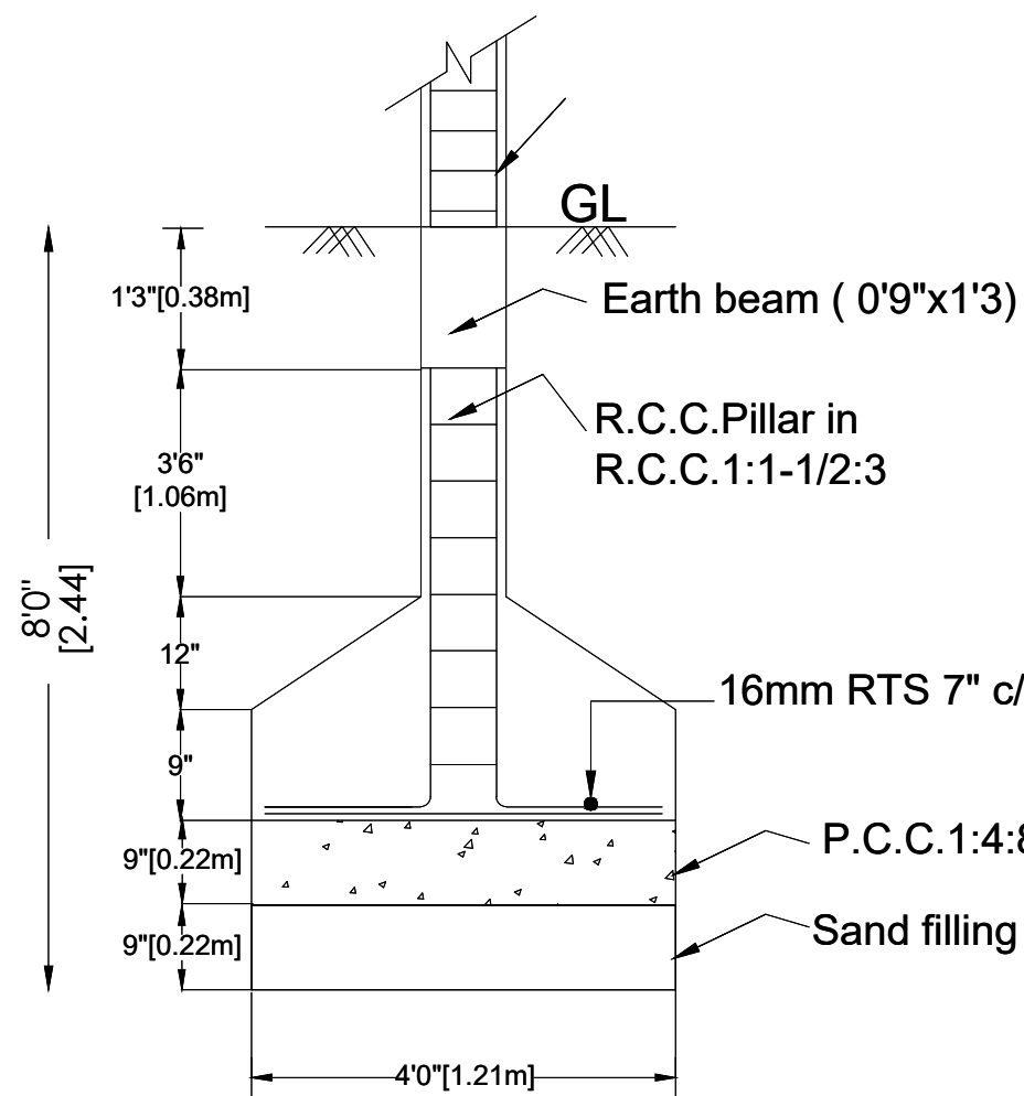
FOUNDATION DETAILS
