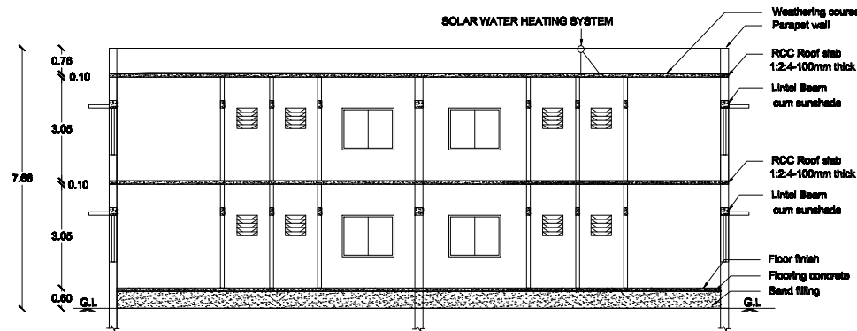
SECTION ON MK
