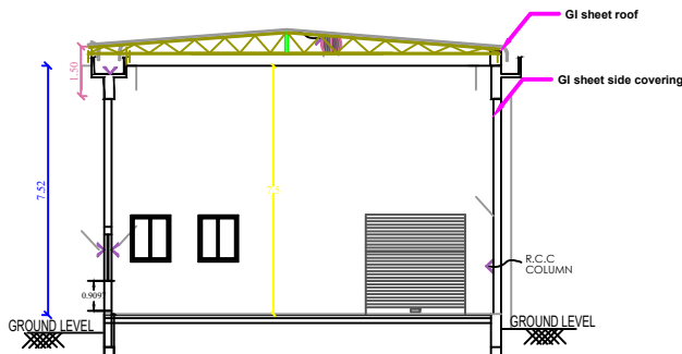
CROSS SECTION ON AB
