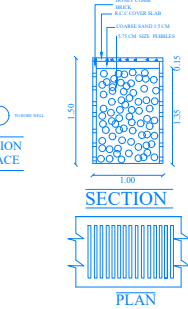
RAIN WATER HARVESTING PERCOLATION BED
