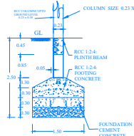
FOUNDATION DETAILS Scale 1:50
