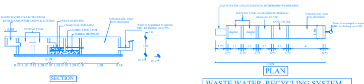
WASTE WATER RECYCLING SYSTEM
