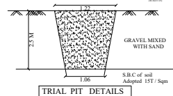
RAIN WATER HARVESTING PERCOLATION BED
