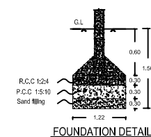
FOUNDATION DETAIL
