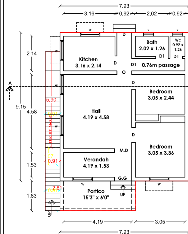
EXI.GROUND FLOOR PLAN
