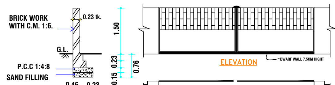
SECTION OF COMPOUND WALL
