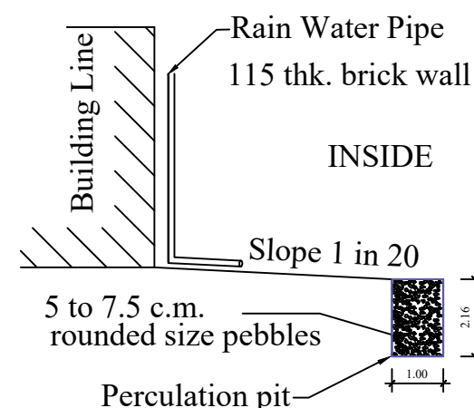
RAIN WATER HARVESTING PERCOLATION PIT RWH_CAPACITY_L=2000LTRS
