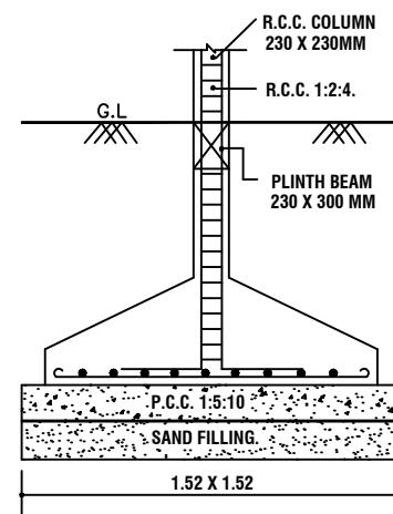
FOUNDATION DETAIL
