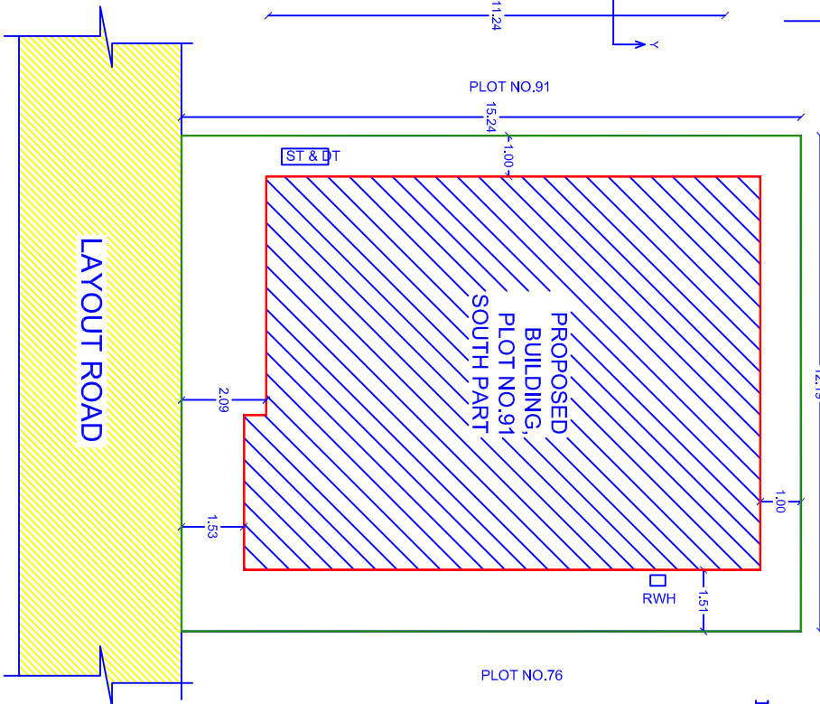
SITE PLAN
