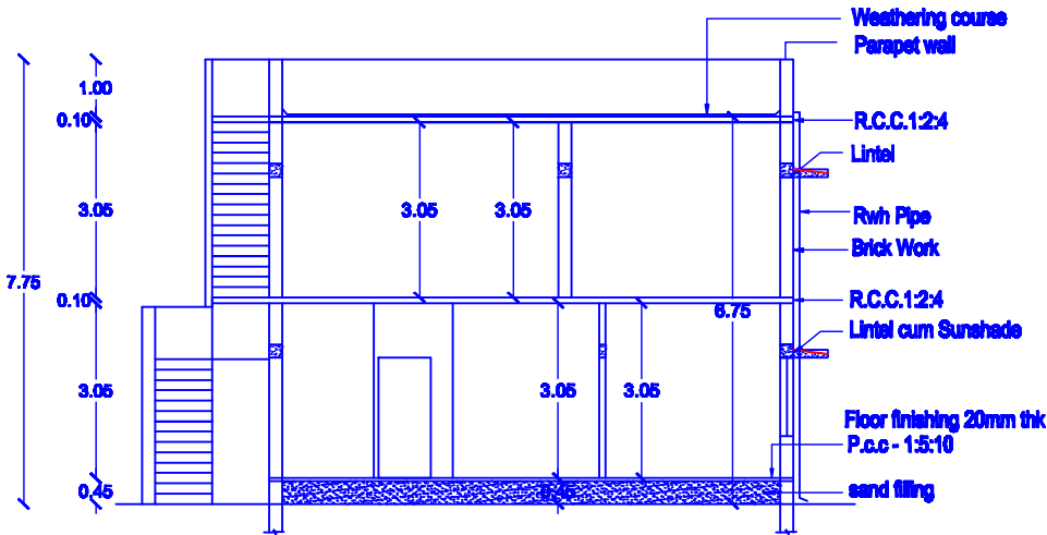
SECTION -XY
