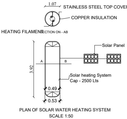
PLAN OF SOLAR WATER HEATING SYSTEM SCALE 1:50
