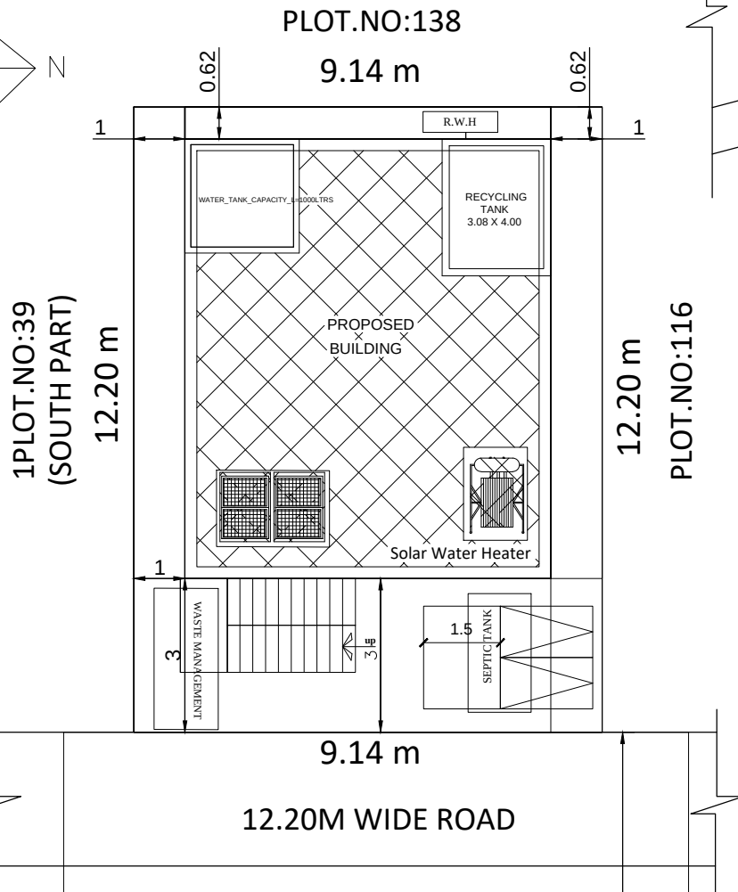
SITE PLAN
