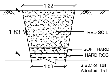
TRIAL PIT DETAILS NOT TO SCALE
