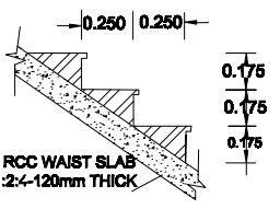
RCC WAIST SLAB 1:2:4-120mm THICK STAIR CASE STEPS SCALE 1:25
