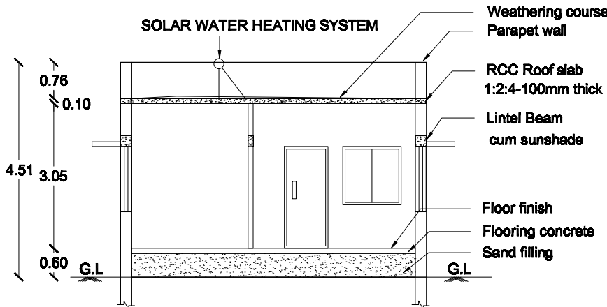
SECTION ON MK
