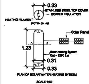
PLAN OF SOLAR WATER HEATING SYSTEM SCALE 1:50
