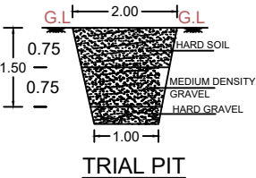
TRIAL PIT
