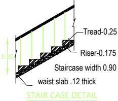
STAIR CASE DETAIL
