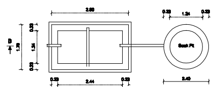
PLAN SEPTIC TANK DETAILS (Scale 1:20)
