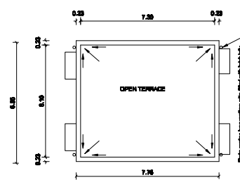
HEAD ROOM TERRACE PLAN
