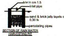
SECTIONAL PLAN OF RAIN WATER HARVESTING PIT SCALE 1:50
