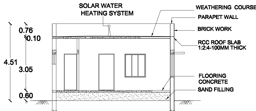
SECTION ON RM
