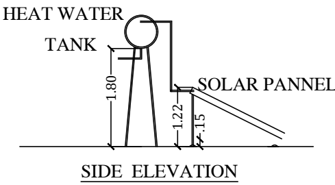
SIDE ELEVATION
