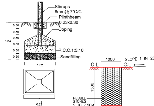
Foundation Details
