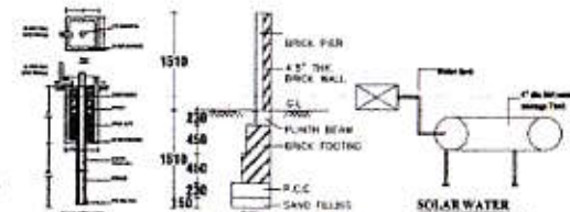
COMPOUND WALL DETAIL SOLAR WATER HEATER SYSTEM
