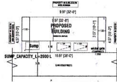
SITE PLAN [1:100]
