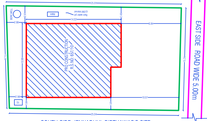
SITE PLAN
