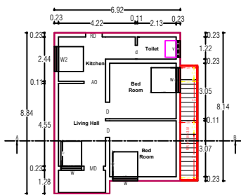
EX.GROUND FLOOR PLAN
