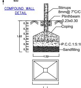
Foundation Details
