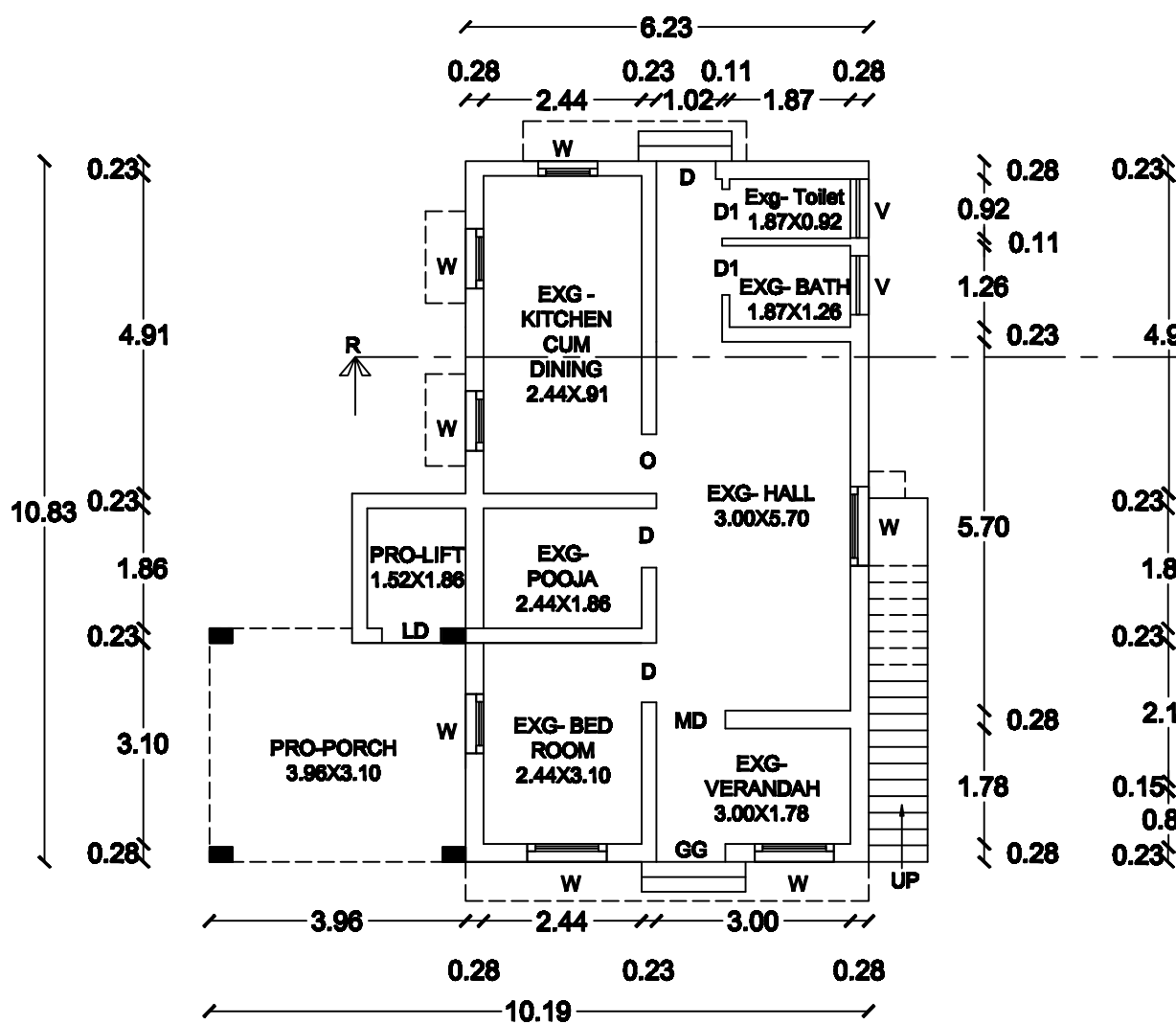
ADDI - GROUND FLOOR PLAN
