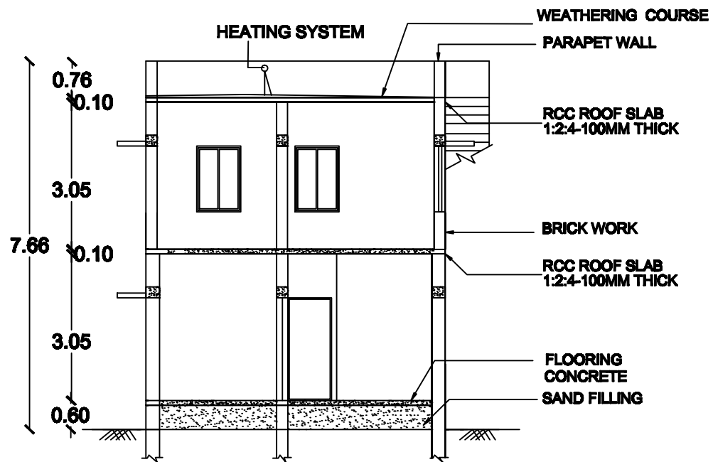
SECTION ON RM
