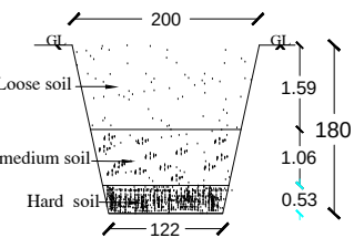
Rain water storage
