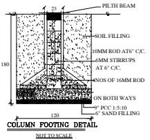
COLUMN FOOTING DETAIL
