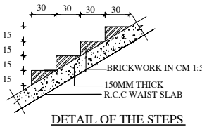
DETAIL OF THE STEPS
