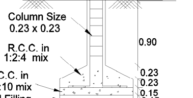
COLUMN DETAILS NOT TO SCALE
