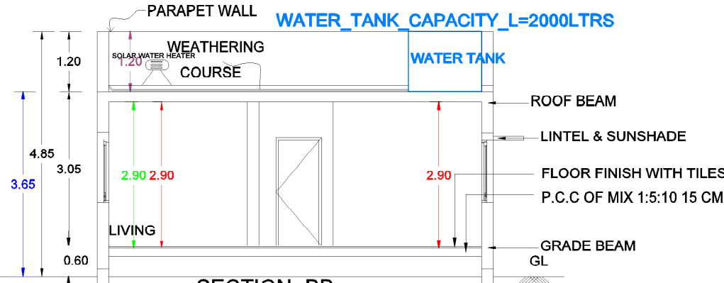
SECTION - BB SECTION
