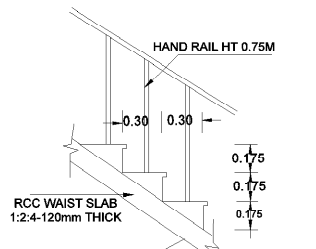
STAIR CASE STEPS SCALE 1:25
