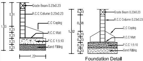
Foundation Details
