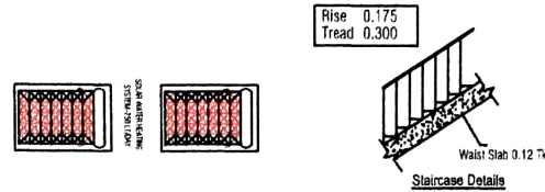
Staircase Details
