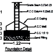
Foundation Detail
