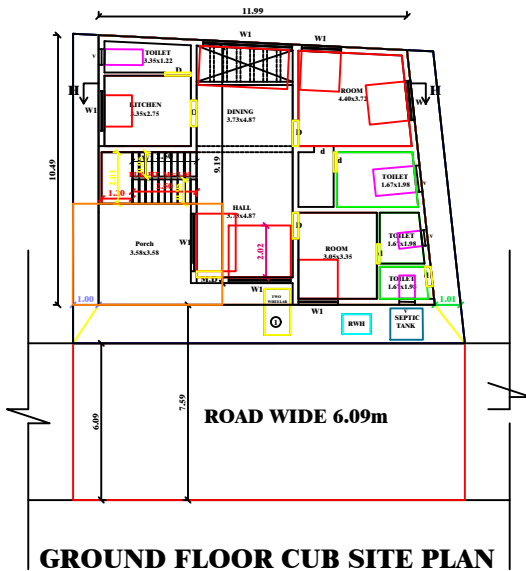
GROUND FLOOR CUB SITE PLAN
